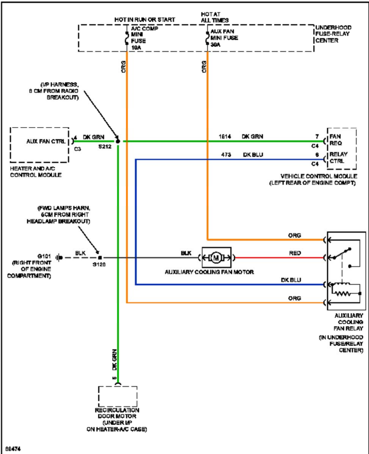
Fig. 15: 5.7L (VIN R), Cooling Fan Circuit
