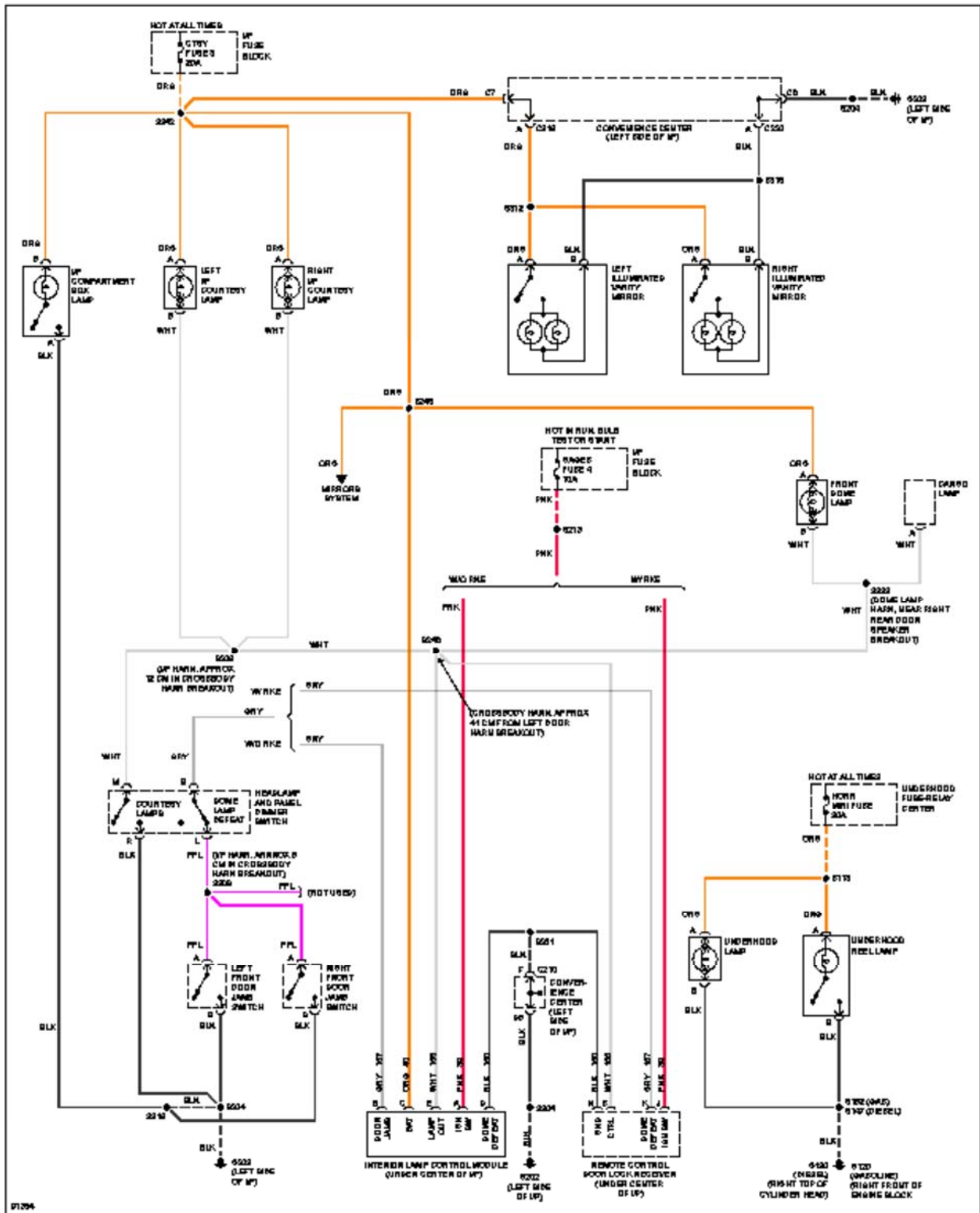
Fig. 53: Courtesy Lamps Circuit, Regular Cab/Extended Cab
