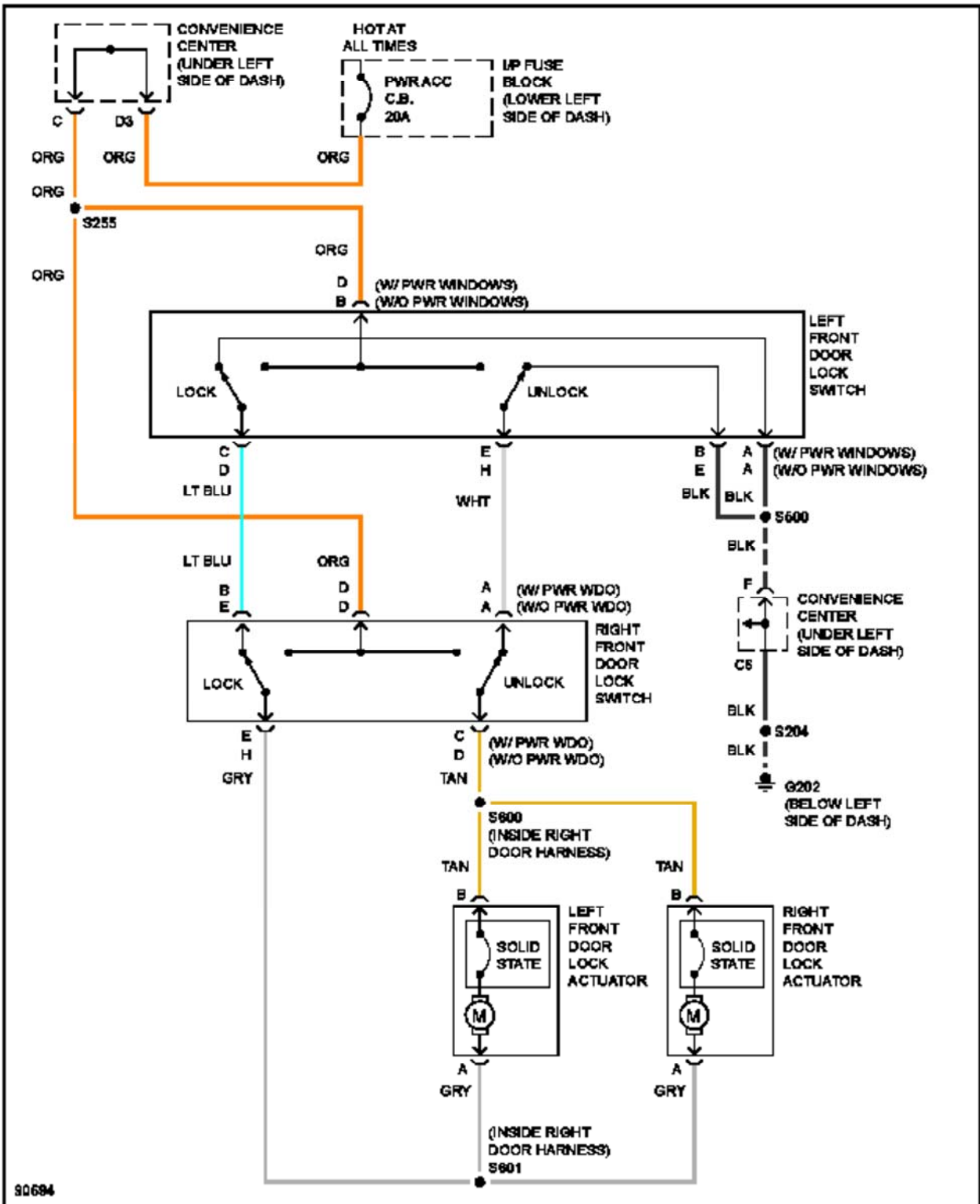
Fig. 60: Door Lock Circuit, W/O Crew Cab
