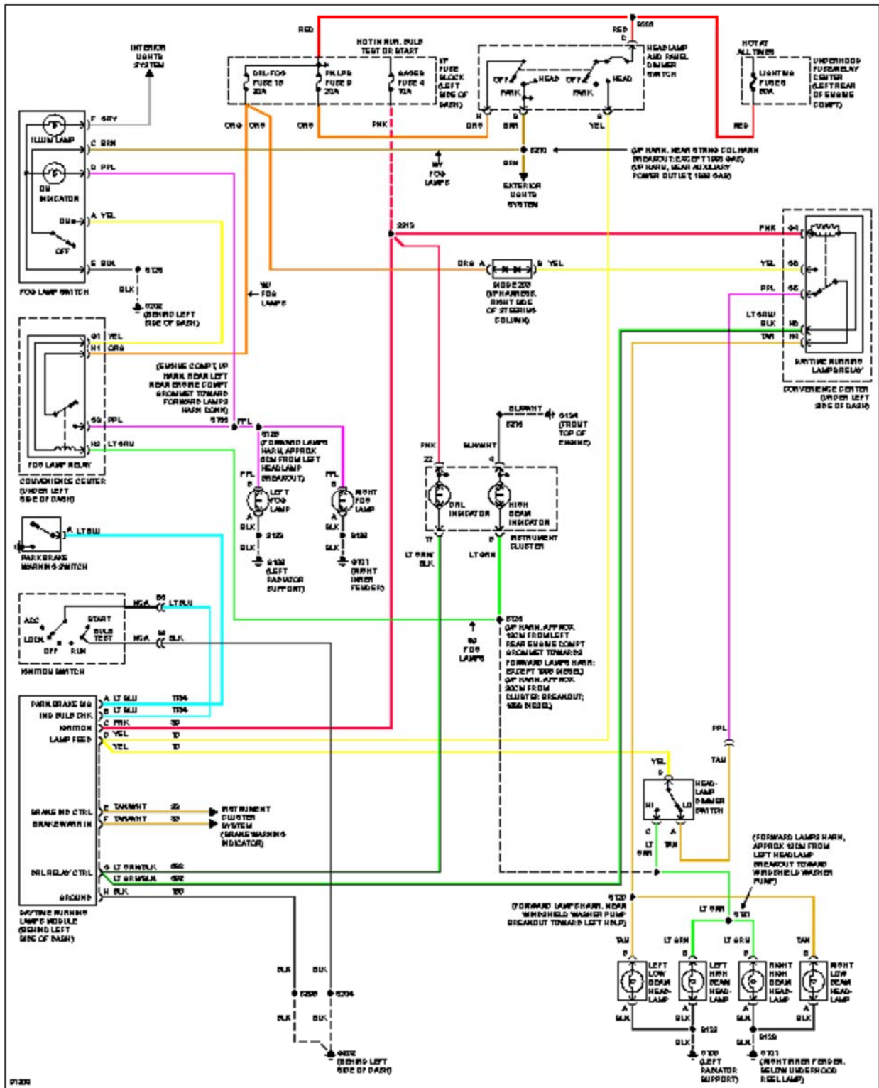
Fig. 45: Headlight Circuit, W/ Quad Headlamps
